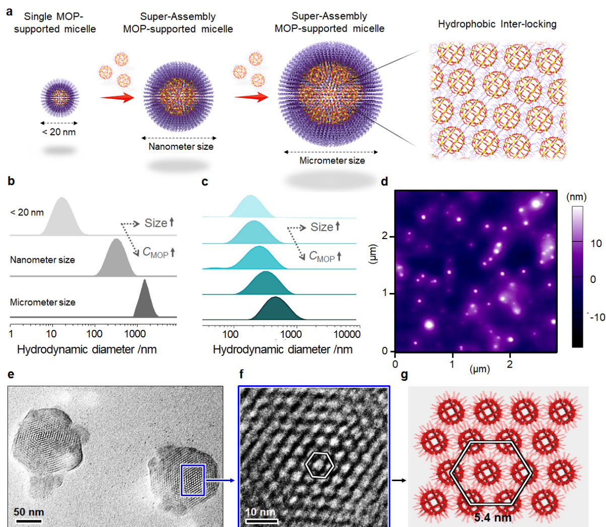
Figure 2. (a) Schematic illustration of the construction of single MOP@micelle and MOP sa @micelles with different size scales. (b) DLS data of Pd 24 L 48 -C 12 MOP-supported micelles with ultrasmall, nanometer, and micrometer sizes. (c) DLS data showing size control of MOP sa @micelles. (d) AFM images of MOP sa @micelles with nanometer size. (e,f) HR-TEM images and (g) simulated structure of the dense packing of Pd 24 L 48 -C 12 MOP in the super-assembly.
