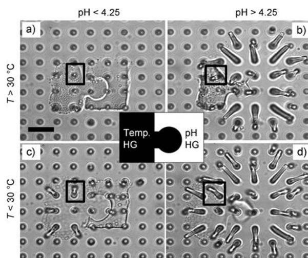
Figure 4. Schematic showing temperature- and pH-responsive hydrogels (HG) fabricated in proximity as interlocking puzzle-piece shapes (center). Optical microscope images at each temperature and pH combination are shown (a–d). The black outline highlights an exemplary post as it is bent at four different angles and directions depending on the combination of conditions. Scale bar: 10 \mu\text{m} .
