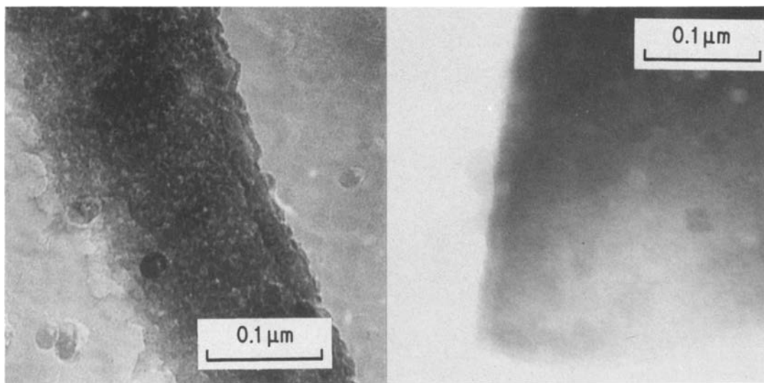
Figure 14 Direct transmission electron micrograph of gel fragments unheated and heated for 12 h at 575° C. Bars indicate 0.1 \mu\text{m} . (Large round features are relics of the underlying carbon film.)
